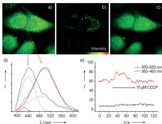
Figure 2. TPM images collected at 360–620 nm (a), 360–460 nm (b), and 500–620 nm (c) of AMg1-AM-labeled (2 μm) Hep3B cells. d) Two-photon-excited fluorescence spectra (normalized) from the hydrophobic (blue) and hydrophilic (red) domains of AMg1-AM-labeled Hep3B cells (λ ex = 780 nm). The cell images shown are representative images from replicate experiments. Gaussian fits are shown in pale blue and brown. e) TPEF intensity collected at 500–620 nm (red) and 360–460 nm (blue) as a function of time.
